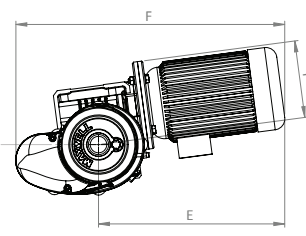
Capstan Versions
